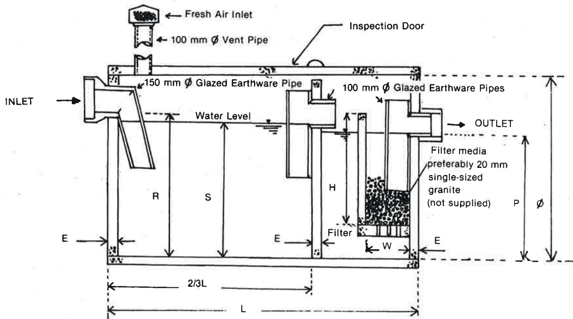
Longitudinal Section — R.C. Septic tank with filter.
