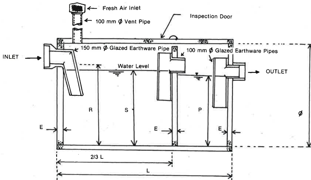
Longitudinal Section — R.C. Septic tank without filter.
