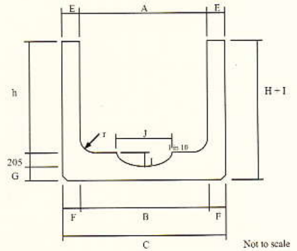
Large Precast R.C. Open Drains Incorporated With A Dry Weather Flow Section
