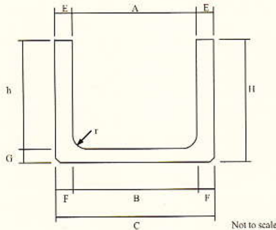
Large Precast R.C. Open Drains
