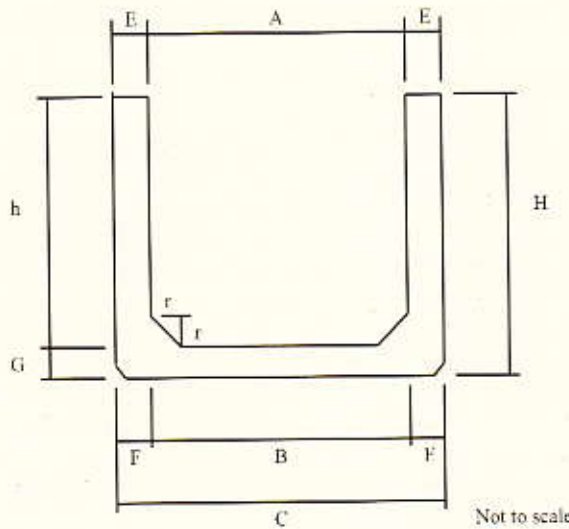
Standard Precast R.C. Open Drains
