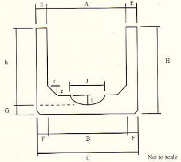
Standard Precast R.C. Open Drains c/w DWF Section
