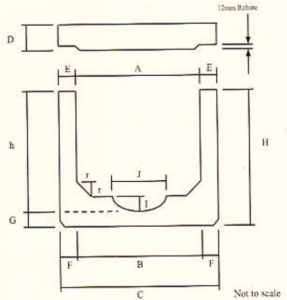
Standard Precast R.C. Box Culverts c/w DWF Section
