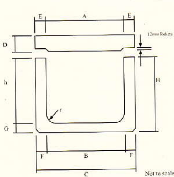
Large Precast R.C. Box Culverts
