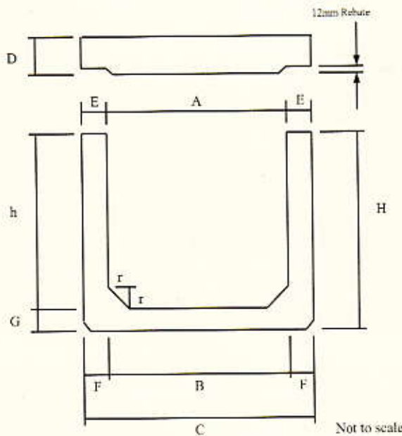
Standard Precast R.C. Box Culverts
