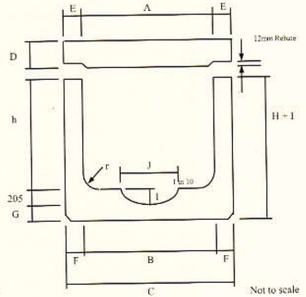
Large Precast R.C. Box Culverts Incorporated With A Dry Weather Flow Section
