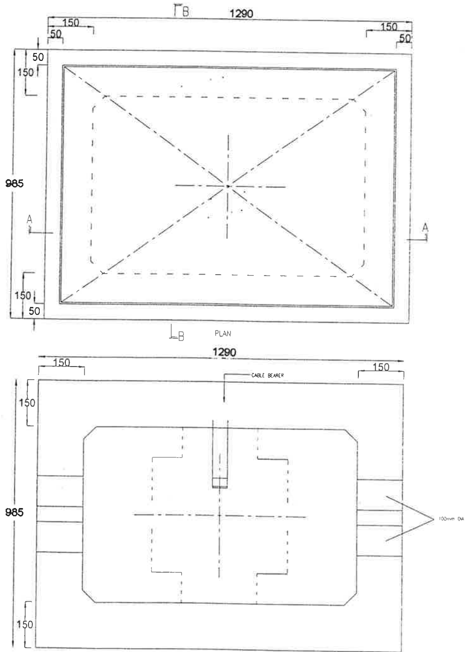
SECTIONAL PLAN C - C JRC7 - JOINT BOX
