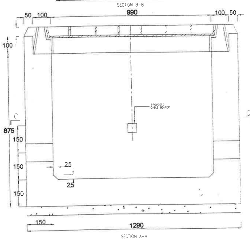
JRC7 - JOINT BOX
