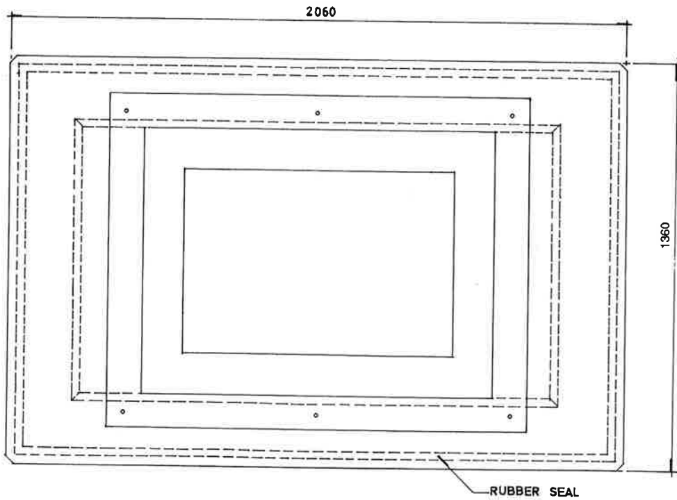
PLAN OF ROOF
