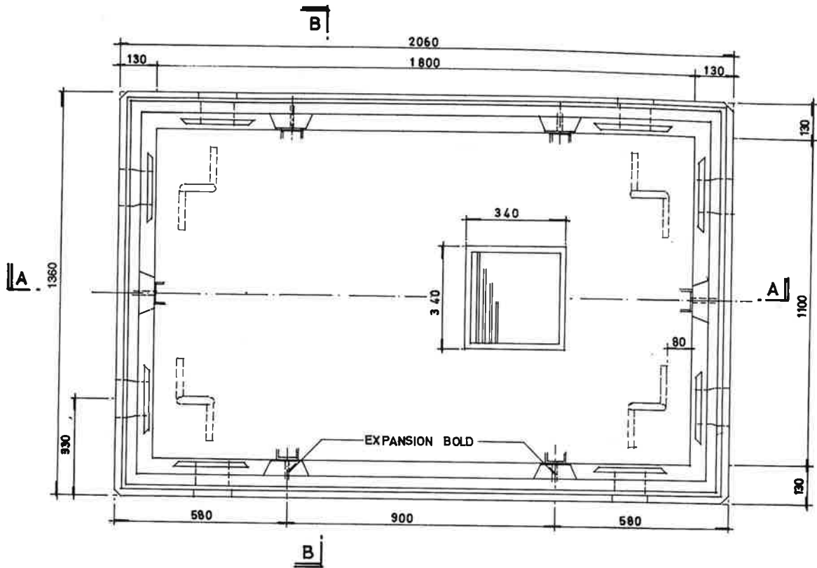
PLAN VIEW OF LOWER SECTION
